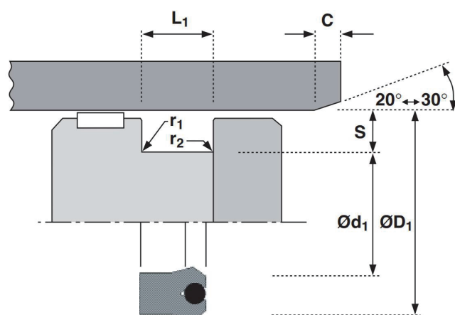
Piston Seal
