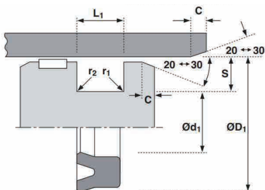
Piston Seal
